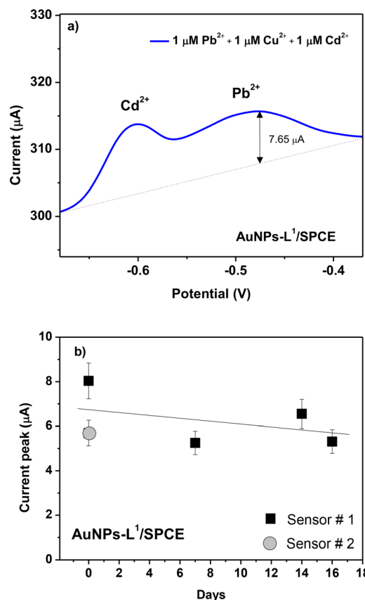
Fig. 12 (a) Selectivity test of the various HMI ions ( Pb^{2+} , Cu^{2+} , and Cd^{2+} ) at 1 μM in seawater and (b) reproducibility test of two AuNPs-L¹/SPCE sensors and signal stability test up to 16 days.
