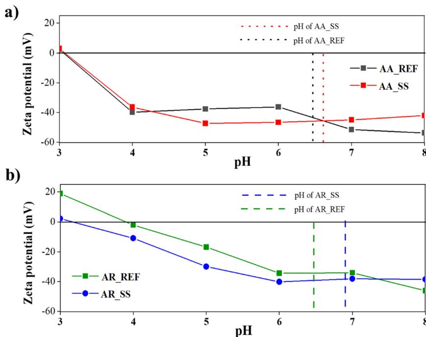
Fig. 5 ZP and IEP of \text{TiO}_2 NPs: a) AA_REF: reference Aldrich Anatase, AA_SS: Aldrich Anatase in soil solution; b) AR_REF: reference Aldrich Rutile, AR_SS: Aldrich Rutile in soil solution.
