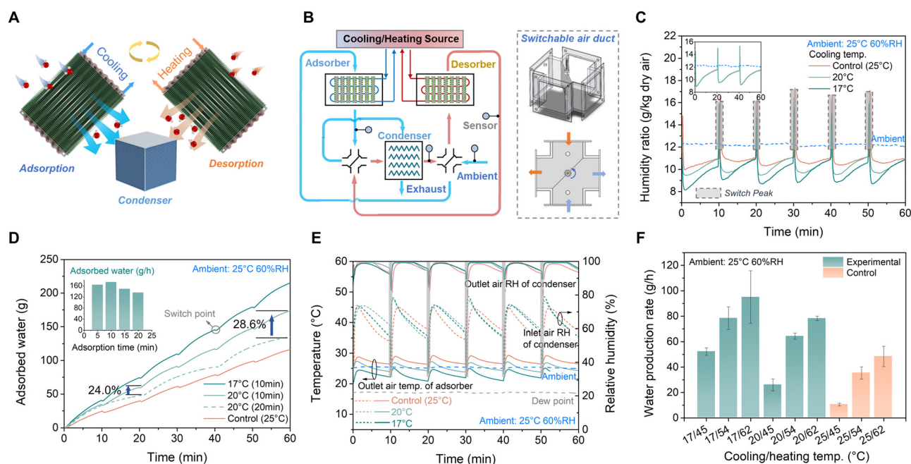
Fig. 2 Water harvesting performance in 25 °C/60%RH. (A) Configurations of the MOF water harvester. (B) Device design of the MOF water harvester. The sorption and desorption airflows can be exchanged by two switchable air ducts. (C) Typical dynamic sorption curves with different cooling temperatures. The humidity ratio refers to the outlet air of the adsorber. (D) Mass variation of adsorbed water. (E) Evolution of temperature and humidity in the condenser. (F) Water production rate with different cooling and heating temperatures. The error bars represent the mean \pm s.d. and the data are determined by the results of six sorption–desorption cycles.
