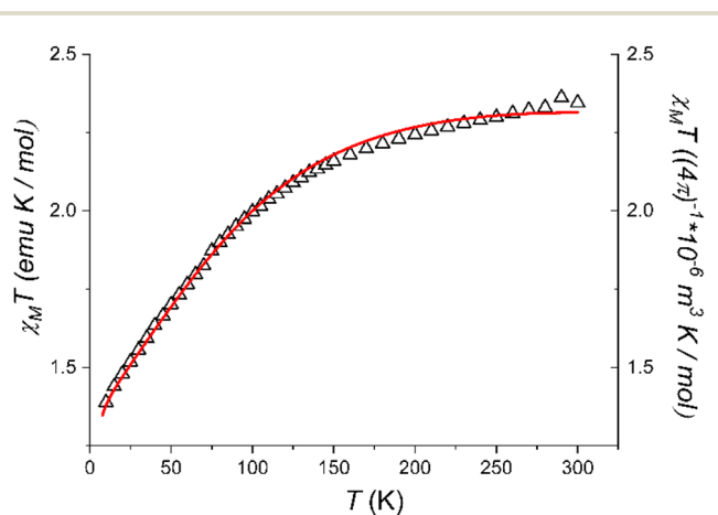
Fig. 3 Temperature evolution of the \chi_{\text{M}}T product of 1 and simulated curve obtained using the parameter-free model reported in the text.
