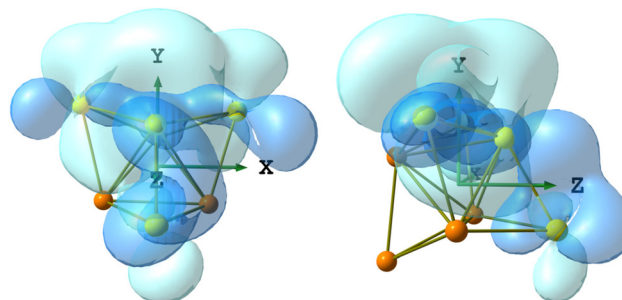
The DFT-optimized structure of 5 is in good agreement with the X-ray data, the RMSD being 0.588 Å. The Ru 4 Au 4 fragments are superimposed in Fig. S34 in the ESI.† The AIM analysis on 5 revealed the presence of three (3,−1) Au–Au BCPs between the Au centre in the axial position of the Ru 4 Au trigonal bipyramid and the three AuPPh 3 fragments capping the Ru 2 Au triangular faces (Fig. 11). The properties at the three BCPs are roughly the same (see the caption of Fig. 11), a result in line with the approximate C 3v symmetry of the Ru 4 Au 4 fragment ( R = 0.077). The values of ρ and V are similar to those obtained for 4-c , suggesting comparable strength of the Au–Au interactions. The presence of bonding overlaps among the Au atoms in 5 can be observed in Fig. 12, where the HOMO is plotted, limited to the contributions of the Au centres.
