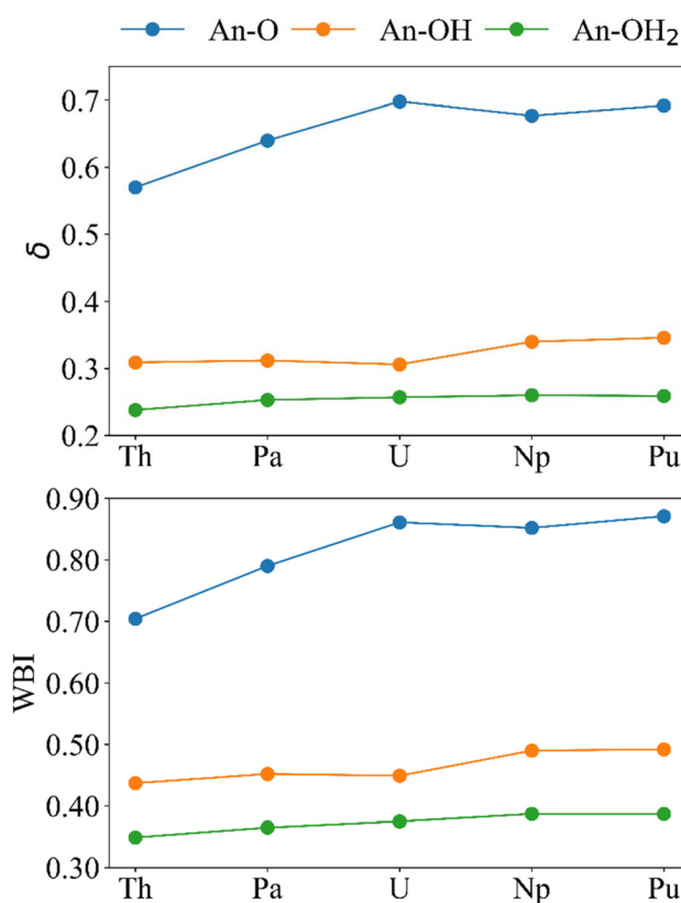
Fig. 6 Bond order metrics for \{[\text{An}(\text{H}_2\text{O})_5]\{\text{Na}(\text{H}_2\text{O})_2\}_5\text{Fe}_{13}\text{O}_{28}\text{H}_{12}\}^{4+} . Upper; delocalisation indices and lower; Wiberg bond indices (calculated at the PBE0/Def2TZVP/SARC-DKH2 level).
