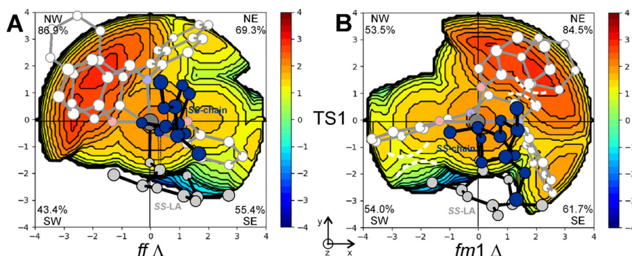
Fig. 5 Steric maps obtained by the % V_{Bur} analysis explaining the wrapping mode energetic preference for ff (A) vs. fm1 (B) configurations in the nucleophilic addition step (TS1) of SS-LA polymerization promoted by the ( R )-1 system. Main steric interactions are reported with dashed lines.
