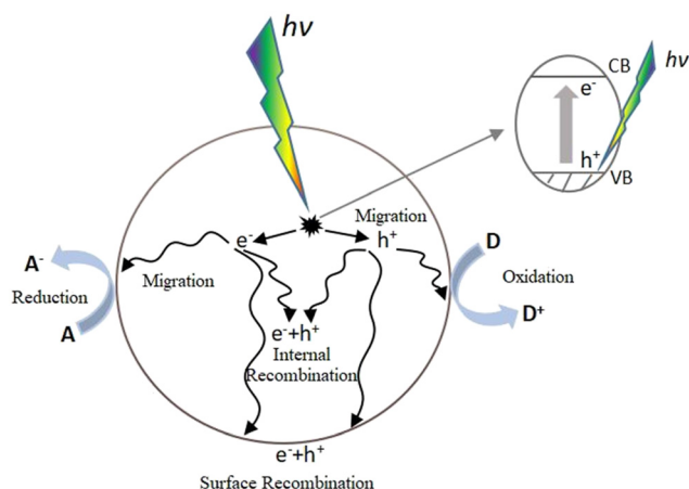
Fig. 1 Photocatalytic process of a semiconductor.
