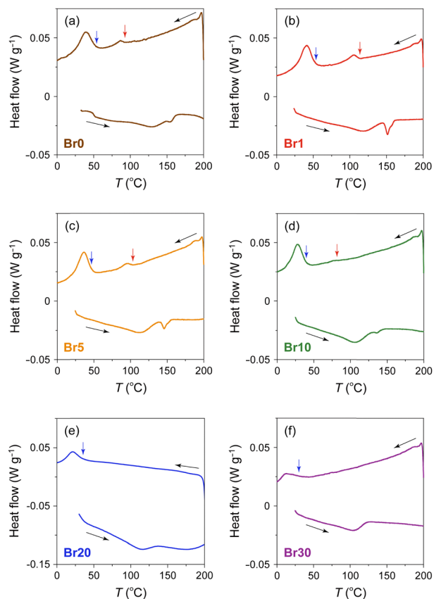
Fig. 3 DSC profiles of AgI-AgBr/MPA composites with various AgI:AgBr molar ratios ((a) Br0 , (b) Br1 , (c) Br5 , (d) Br10 , (e) Br20 , and (f) Br30 ). The red and blue arrows indicate the onset temperatures of the transition on the high- and low-temperature sides, respectively, in the cooling process.
