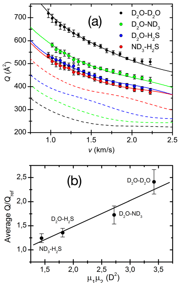
Fig. 8 (a) Total integral collision cross-sections Q(v) , as a function of the collision velocity v , for the D 2 O–D 2 O, D 2 O–ND 3 , D 2 O–H 2 S and ND 3 –H 2 S polar pairs. The dashed lines are Q_{ref}(v) calculated for the reference pairs, Ar–Ar (black, reference for D 2 O–D 2 O), Ar–Kr (green, reference for D 2 O–ND 3 ), Ar–Xe (blue, reference for D 2 O–H 2 S) and Kr–Xe (red, reference for ND 3 –H 2 S) and convoluted in the laboratory frame under the same conditions. (b) Average ratios of the polar pairs cross-sections versus the reference systems as a function of the permanent dipole product of the polar pairs. 1 D (Debye) = 3.336 \times 10^{-30} C-m. Reproduced from ref. 44 with permission from AIP publishing, copyright © 2014.
