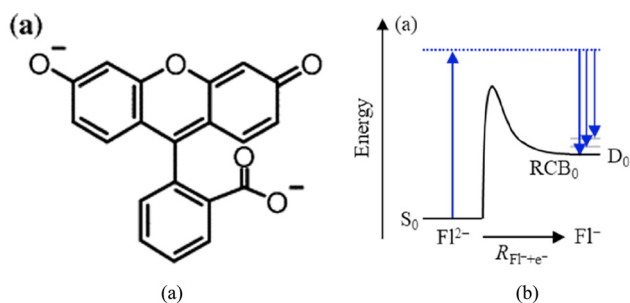
Fig. 7 Structure of doubly deprotonated fluorescein \text{F}^{2-} (a) and depiction of repulsive Coulomb barrier connecting \text{F}^{2-} to singly deprotonated \text{FI}^{1-} (b). Reprinted from Fig. 7 of ref. 2 (a) and Fig. 8 of ref. 2 (b) with permission of the American Chemical Society (2023).
