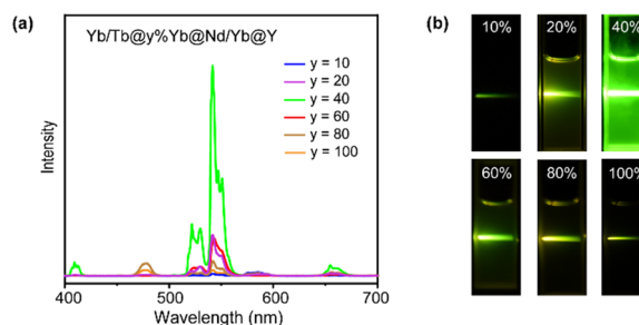
Fig. 3 (a) Upconversion luminescence spectra of Tb/Yb@ y\% Yb@Nd/Yb@Y ( y = 10\text{--}100 ) CSSS NPs. (b) Digital photos of Tb/Yb@ y\% Yb@Nd/Yb@Y ( y = 10\text{--}100 ) CSSS NPs.
