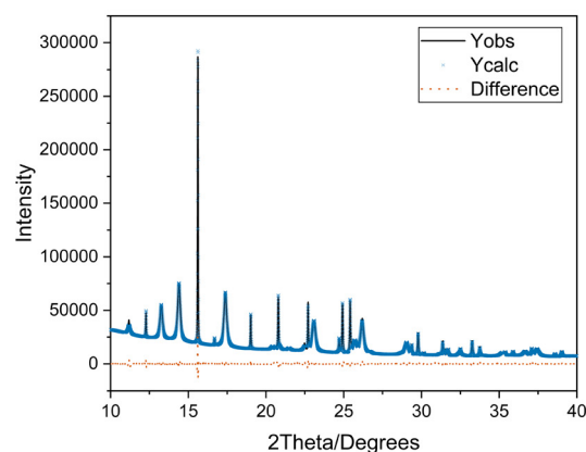
Fig. 2 (a) Crystal structures of calcite (left) and vaterite (right), where green is calcium, black is carbon and red is oxygen. Both crystal structures are orientated in the same direction to highlight the difference between the a and c lattice parameters. The vaterite structure shown is a simplified version of the Kamhi structure, 33 removing the disorder to facilitate comparison. (b) Diffraction pattern for sample 68-08 with the observed and calculated data and the difference.
