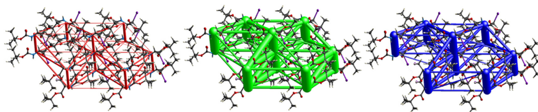
Fig. 26 Energy frameworks for electrostatic (red), dispersion (green) and total interaction energies (blue) for a cluster of nearest-neighbour molecules in Boc-Ala(3-I)-O t Bu (6). The energy tube size is 200, and the energy threshold is 0 \text{kJ mol}^{-1} .
