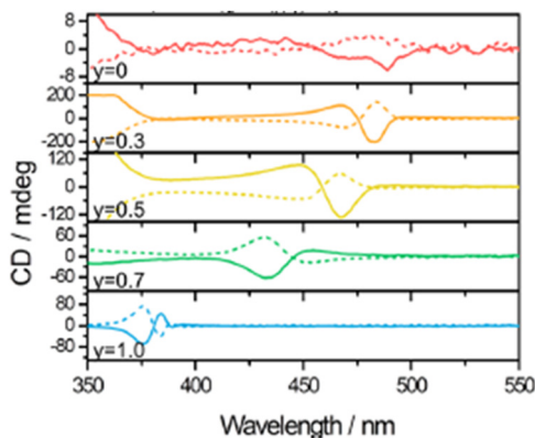
Fig. 18 CD spectra of (R/S\text{-NEA})_2\text{Pb}_{14(1-y)}\text{Br}_{4y} . Reprinted with permission from ref. 23 Copyright©2020 American Chemical Society.
