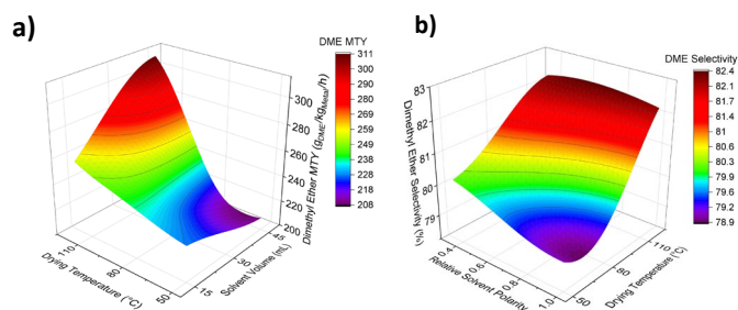
Fig. 2 Three-dimensional response surface model showing the impact of a) drying temperature and solvent volume on predicted DME metal time yield and b) relative solvent polarity and drying temperature on predicted DME selectivity.
