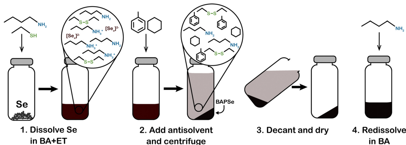
Fig. 13 Schematic for a precipitation-based procedure for isolating alkylammonium polyselenides from a solution of butylamine (BA) and ethanethiol (ET). This same procedure can also be applied to isolating metal organics from amine–thiol solutions. Reprinted with permission. 35 Copyright 2023 Royal Society of Chemistry.
