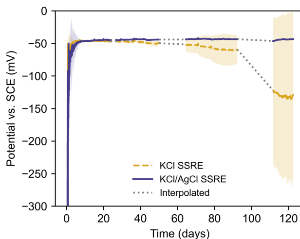
Fig. 5 long term potential monitoring of KCl SSRE and KCl/AgCl SSREs in 1 \text{ g L}^{-1} \text{Na}_2\text{S} solution in pH 9 buffer. Mean potentials ( n = 5 ) are reported with the coloured shading indicating the 95% confidence interval. Interpolated sections indicate periods where the conventional SCE reference suffered sulphide poisoning.
