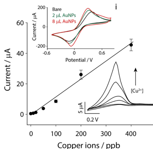
Fig. 2 Calibration curve for copper ions in a standard solution, i.e. 0.1 M HCl, obtained by modifying the electrochemical strips with 2 μL of AuNPs. Experimental parameters: E_{\text{dep}} = -0.4 V; t_{\text{dep}} = 300 s; E_{\text{begin}} = 0.1 V; E_{\text{end}} = 0.6 V; E_{\text{step}} = 0.01 V; scan rate = 0.5 V s -1 . The voltammetric curves relating to the measured concentrations for copper are also reported. Inset i: Cyclic voltammograms for the evaluation of the optimal amount of AuNPs, between 2 and 8 μL. The measurements were conducted in triplicate in the presence of 5 mM potassium ferricyanide in a 0.1 M potassium chloride solution.
