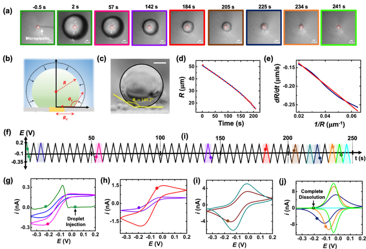
Fig. 3 (a) Optical micrographs recorded during the dissolution of a 51 \mu\text{m} radius droplet containing 155 \mu\text{M} of (\text{Cp}^*)_2\text{Fe}^{\text{II}} in a 10 \text{ mM} \text{NaClO}_4 aqueous bulk phase. The solid red line incrustated in the micrographs indicates the position of the gold-disk electrode. The scale bar is 10 \mu\text{m} . (b) Side-view schematic of the droplet sitting on the electrode. (c) Side-view optical micrograph of a DCE droplet on a glass surface and immersed in water. The scale bar represents 10 \mu\text{m} . (d) Apparent droplet's radius as a function of time measured from the optical micrographs in (a). The data points shown in red represent the apparent radius of the droplet measured using the acquired micrographs. The solid blue curve represents a polynomial fit used to obtain a smooth representation of the data points. (e) Normal velocity of the water|DCE as a function of the inverse of the droplet's radius. The solid navy curve is a linear fit on the data, slope = -2.4 \pm 0.003 \text{ cm}^2 \text{ s}^{-1} , R^2 = 0.992 . (f) Potential ramp applied during the dissolution of the droplet shown in (a). The colored segments in the potential ramp function correspond to the colored segments of the voltammogram in (g)–(j). Panels (g)–(j) show cyclic voltammograms recorded simultaneously with the optical micrographs during the dissolution of the DCE droplet at a scan rate of 0.2 \text{ V s}^{-1} . The color code used for the cyclic voltammograms matches the color code in (f). The points on the cyclic voltammogram indicate the exact time when the frames in (a) were taken. The voltammograms were smoothed using adjacent weighted averaging with 19 points per window and a Savitzky–Golay algorithm with 32 points per window, and a periodic boundary condition. See Fig. S4† for an overlay of experimentally obtained CV and noise filtered CV of the purple curve in (h).
