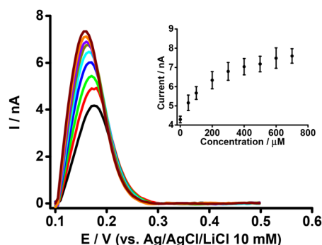
Fig. 5 DPVs at different concentrations of \beta -CD at fixed concentrations of BSA (0.6 mM) and PFOA ( 50 \mu\text{M} ) at the \mu\text{TIES} array. Cell composition as given in Scheme 1. Black, red, green, blue, cyan, dark yellow, violet, orange, and wine red, respectively, represent the DPVs at 50, 100, 200, 300, 400, 500, 600, and 700 \mu\text{M} \beta -CD. Inset: relationship between peak current and concentration of \beta -CD. DPVs were background-subtracted followed by baseline-corrected. Error bars indicate \pm 1 standard deviation from two independent measurements.
