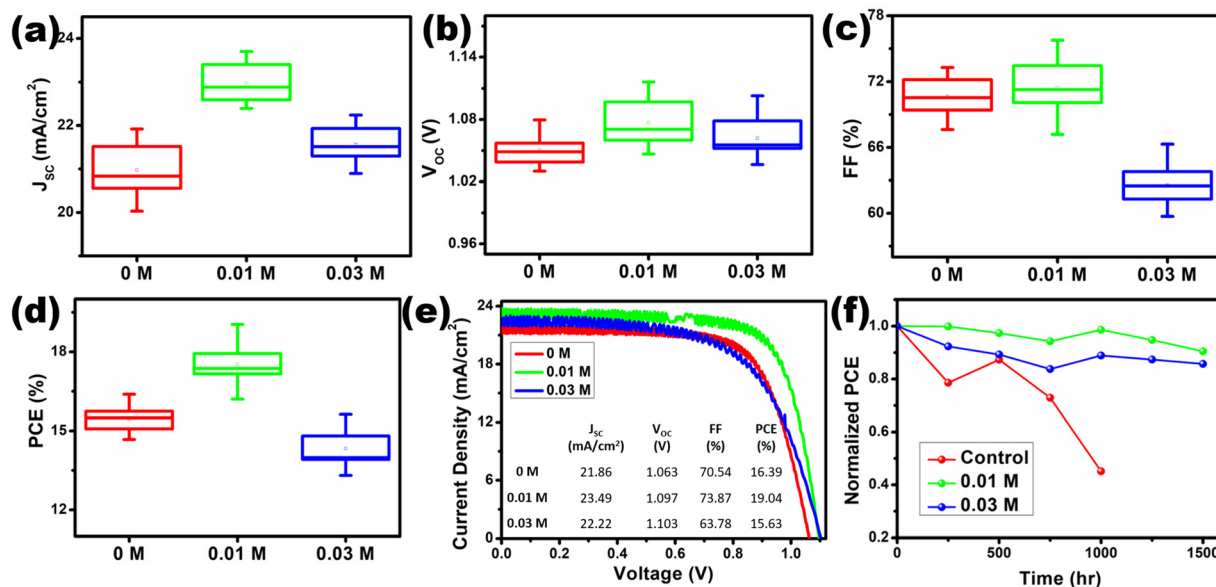
Fig. 7 Box chart of (a) J_{SC} , (b) V_{OC} , (c) FF, and (d) PCE of the [TMPA][TFSI] ionic liquid-modified PSCs. (e) J - V curve of the most efficient cells for different [TMPA][TFSI] ionic liquid modification. (f) Stability comparison of control and [TMPA][TFSI] ionic liquid-modified devices.
