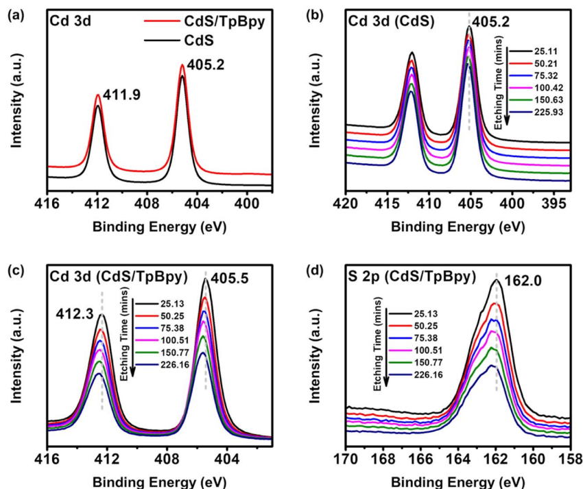
Fig. 2 (a) Cd 3d XPS spectra at the surface of CdS/TpBpy-20% and CdS. (b) Cd 3d high resolution XPS spectra of CdS at different etching times. (c) Cd 3d and (d) S 2p high resolution XPS spectra of CdS/TpBpy-20% at different etching times.
