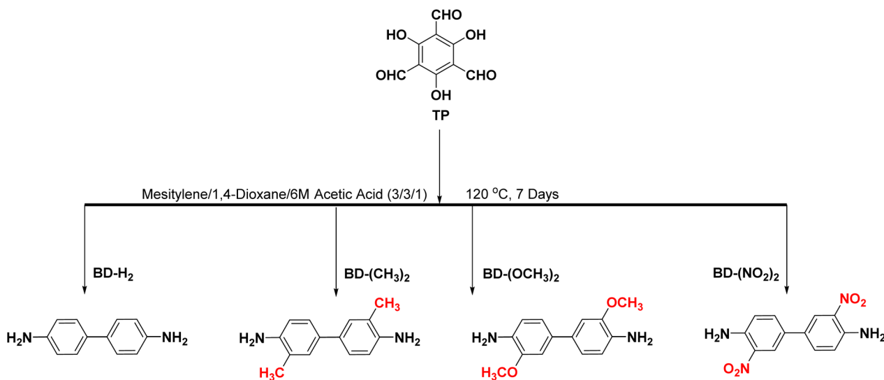
Fig. 8 Schematic diagram of the synthetic path for TpBD-X [X = \text{H}_2 , \text{-(CH}_3\text{)}_2 , \text{-(OCH}_3\text{)}_2 , and \text{-(NO}_2\text{)}_2 ].
