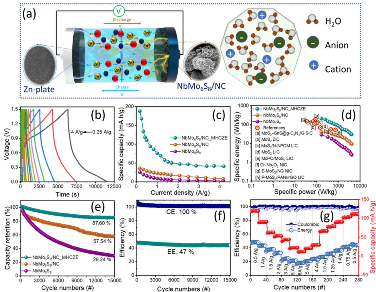
Fig. 5 (a) Schematic of the \text{NbMo}_6\text{S}_8/\text{NC} ZIC construction and working mechanism. (b) Charge–discharge profiles of the \text{NbMo}_6\text{S}_8/\text{NC} electrode in MHCZE electrolyte. (c) Specific capacity, (d) Ragone plot, and (e) long-term cycling capacity retention at a current density of 2.5 \text{ A g}^{-1} for \text{NbMo}_6\text{S}_8 and \text{NbMo}_6\text{S}_8/\text{NC} ZICs. (f) Coulombic and energy efficiencies, and (g) a capability test at different current densities for the \text{NbMo}_6\text{S}_8/\text{NC} electrode in MHCZE electrolyte.
