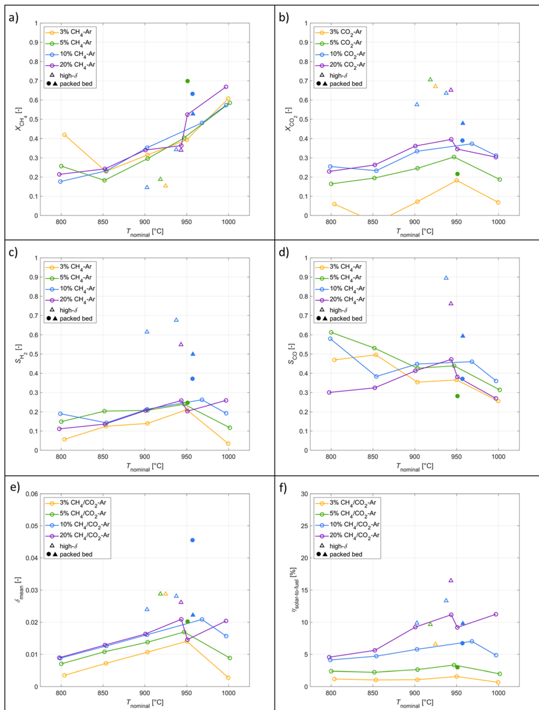
Fig. 7 Experimental results as a function of the nominal temperature for redox reforming cycles: (a) CH 4 molar conversion for the reduction step. (b) CO 2 molar conversion for the oxidation step. (c) H 2 selectivity of the reduction step. (d) CO selectivity of the reduction step. (e) Average \delta of CeO 2- \delta across a complete redox reforming cycle. (f) Solar-to-fuel energy efficiency. Tests were performed at varying inlet reacting gas concentrations (3%, 5%, 10%, 20%), high- \delta cycles, and with the packed bed installation in the tubular section.
