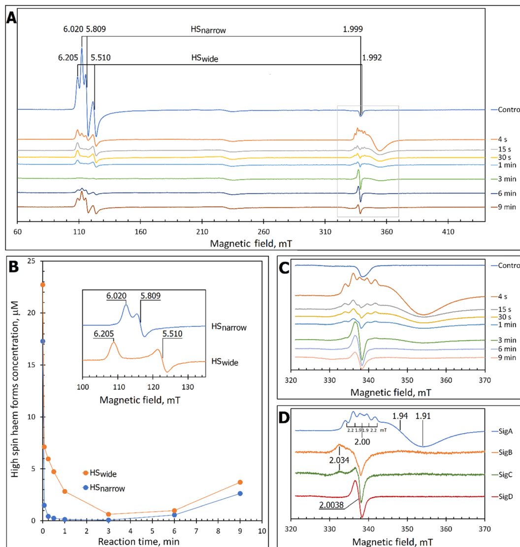
Fig. 2 X-band CW EPR spectroscopy of DtpAa upon reaction with \text{H}_2\text{O}_2 at 10 K and pH 5.0. (A) The EPR spectra of DtpAa before (Control) and at different times after mixing with 400 \mu\text{M} \text{H}_2\text{O}_2 . The g -values of the two HS ferric heme forms, \text{HS}_{\text{narrow}} and \text{HS}_{\text{wide}} , are indicated and are consistent with those previously reported. 36 The signal at ~230 millitesla is a background contribution. (B) The kinetic dependences averaged over two independent experiments of the two HS ferric heme forms. The inset gives the respective line shapes of the two HS signals, in the g = 6 region, extracted by spectral subtraction with variable coefficient, 48 formulated as follows: \text{HS}_{\text{narrow}} = (\text{Control}) - 3.3 \times (4 \text{ s}) ; \text{HS}_{\text{wide}} = (4) - 0.084 \times (\text{Control}) . (C) Detailed view of the spectral region covering the field interval of 320–370 mT within the grey frame in (A). All instrumental conditions used were the same as in (A) (see Experimental section) but with a slower R_s = 0.325 \text{ mT s}^{-1} . (D) The spectral components (pure line shapes) contributing to the EPR spectra shown in C. All signals (SigA to SigD) were obtained by using the procedure of spectra subtraction with variable coefficient, 48 formulated as follows; SigA = (4 \text{ s}) - 0.23 \times (\text{Control}) ; SigB = (15 \text{ s}) - 0.61 \times (4 \text{ s}) - 0.145 \times (1 \text{ min}) ; SigC = (1 \text{ min}) - 0.61 \times (4 \text{ s}) - 0.392 \times (15 \text{ s}) ; SigD = (6 \text{ min}) - 0.337 \times (3 \text{ min}) . The g -values of spectral points of interest are indicated and the distances between the hyperfine components of SigA, are indicated in millitesla.
