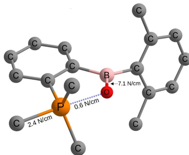
Fig. 2 Selected relaxed force constants in 2 computed at the \omega\text{B97XD}/\text{def2-tzvp} level of theory. All hydrogen atoms as well as the 2,4,6- iso - \text{Pr}_3\text{C}_6\text{H}_2 moieties are omitted for clarity. The coupling force constant between the P–O interaction and the opposing P–C bond is synergistic (note the negative sign) and pronounced at -0.20 \text{ N cm}^{-1} .
