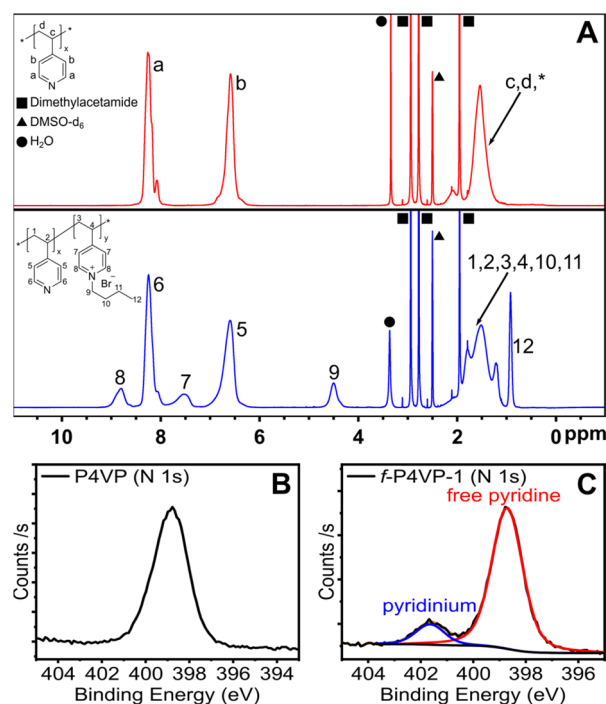
Fig. 4 Characterization of the polymer product synthesized under continuous flow. (A) ^1\text{H} NMR spectra of P4VP (top, red) and f -P4VP-1 (bottom, blue) in DMSO- d_6 . (B). XPS N 1s spectrum of P4VP. (C). XPS N 1s spectrum of f -P4VP-1. Analysis reveals two distinct N species at 398.71 eV and 401.64 eV, corresponding to free pyridine and quaternized pyridinium on the polymer, respectively. Samples were isolated from solutions in DMAc prior to NMR and XPS analysis.
