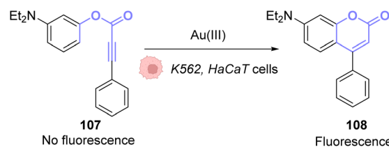
Fig. 36 Gold(III)-catalysed hydroarylation of non-fluorescent 107 into a fluorescent coumarin. 87
