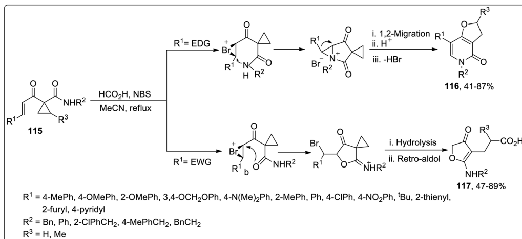
Scheme 36 Synthesis of dihydrofupyrinones 116 and 3(2H)-furanones 117 via Cloke-Wilson rearrangement.
