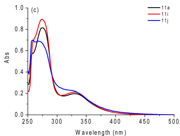
Fig. 3 Comparative absorption UV-vis spectra (concentration at 50 \mu\text{M} ) of compounds 11a (Se atom), 11i (S atom) and 11j (Te atom) in (a) DCM, (b) ACN and (c) DMSO, respectively.
