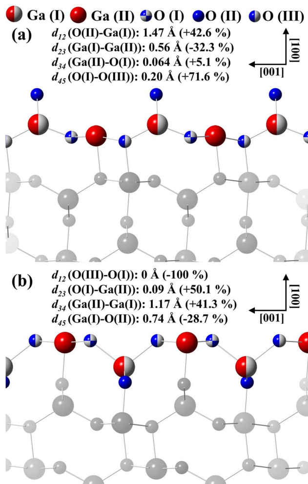
Fig. 9 Interlayer distances calculated for the models with termination (a) A and (b) B proposed to describe the \beta -Ga 2 O 3 (100) surfaces.
