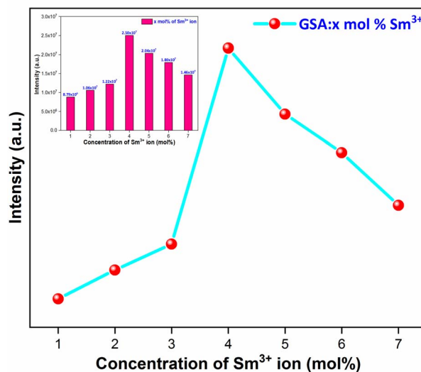
Fig. 14 Relative PL intensity of \text{Gd}_{1-x}\text{Sr}_2\text{AlO}_5:x\text{Sm}^{3+} ( x = 1-7 mol% \text{Sm}^{3+} ) phosphors and inset represent the intensity of respective samples.
