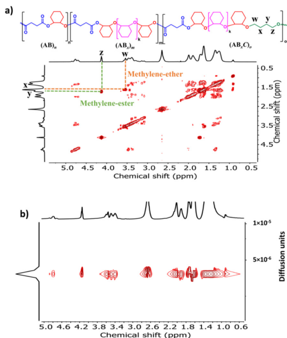
Fig. 7 COSY and DOSY-NMR spectra (600 MHz, \text{CDCl}_3 , 30 ^\circ\text{C} ) of the copolymer from ROCOP of SA, CHO and THF using a SA/CHO/THF/ \text{SnOct}_2 molar ratio of 50 : 150 : 150 : 1 (Table 2, entry 3).
