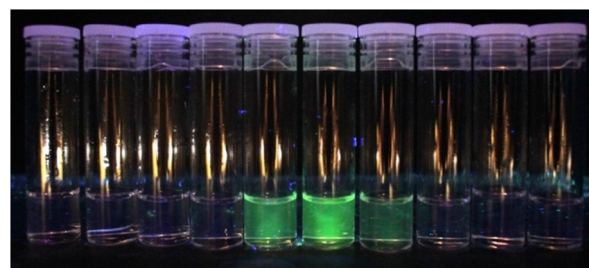
Fig. 3 Eluted GPC solvent showing the emission from the yellow (green-emissive) Nap-PA-CHO polymer in vials 5–7 ( t_R = 14\text{--}17 min; each vial = 1 min, i.e. 1 mL).
