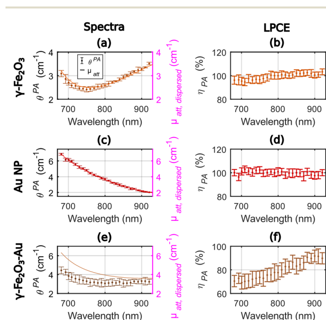
Fig. 4 Photoacoustic and attenuation spectra ((a), (c) and (e)) and Light-to-Photoacoustic Conversion Efficiency (LPCE, (b), (d) and (f)) for the maghemite nanoflowers ( \gamma\text{-Fe}_2\text{O}_3 ), the gold nanoparticles (Au NP) and the maghemite nanoflowers decorated with gold nanoparticles ( \gamma\text{-Fe}_2\text{O}_3\text{-Au} ), respectively. The photoacoustic coefficients \theta^{\text{PA}} were obtained with a calibrated photoacoustic spectrometer. Here, \theta^{\text{PA}} is assumed to be equal to the photothermal conversion efficiency multiplied by the absorption coefficient of the dispersed phase. The attenuation coefficient \mu_{\text{att, dispersed}}(\lambda) is measured with a spectrophotometer. The LPCE is the ratio of \theta^{\text{PA}} to \mu_{\text{att, dispersed}}(\lambda) . For the photoacoustic coefficients, the median \pm median absolute deviation values were displayed with dot markers and error bars. For the LPCE, the error bars correspond to the relative uncertainty and consider all the measurement and calibration steps. The axis ranges for the LCPE were 40%.
