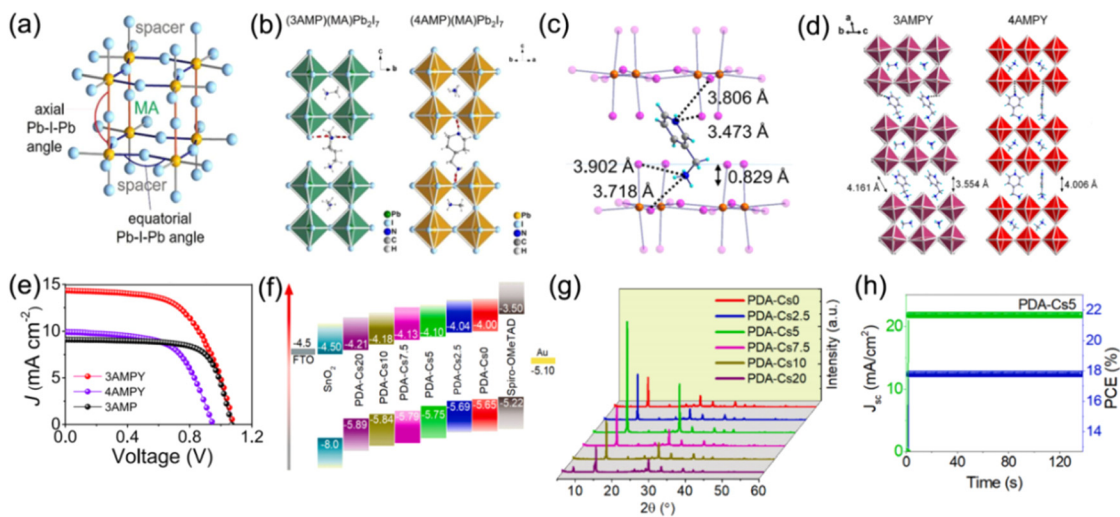
Fig. 6 (a) Schematic diagram of axial and equatorial Pb–I–Pb angles for 3AMP and 4AMP based DJ perovskites. (b) Structures of (3AMP)(MA)Pb 2 I 7 and (4AMP)(MA)Pb 2 I 7 . Reproduced with permission from ref. 33. Copyright 2018 American Chemical Society. (c) Distance between organic cations and inorganic frameworks for (3AMPY)(MA)Pb 2 I 7 . (d) Structures of (3AMPY)(MA)Pb 2 I 7 and (4AMPY)(MA)Pb 2 I 7 . (e) J – V results of 3AMPY, 4AMPY and 3AMP based DJ PSCs. Reproduced with permission from ref. 74. Copyright 2019 American Chemical Society. (f) Energy band alignment and (g) XRD patterns of (PDA)C s x (MA) 3– x Pb 4 I 13 films. (h) Stabilized PCE and J sc values of the champion (PDA)C s 0.05 (MA) 2.95 Pb 4 I 13 device. Reproduced with permission from ref. 78. Copyright 2022 Elsevier.
