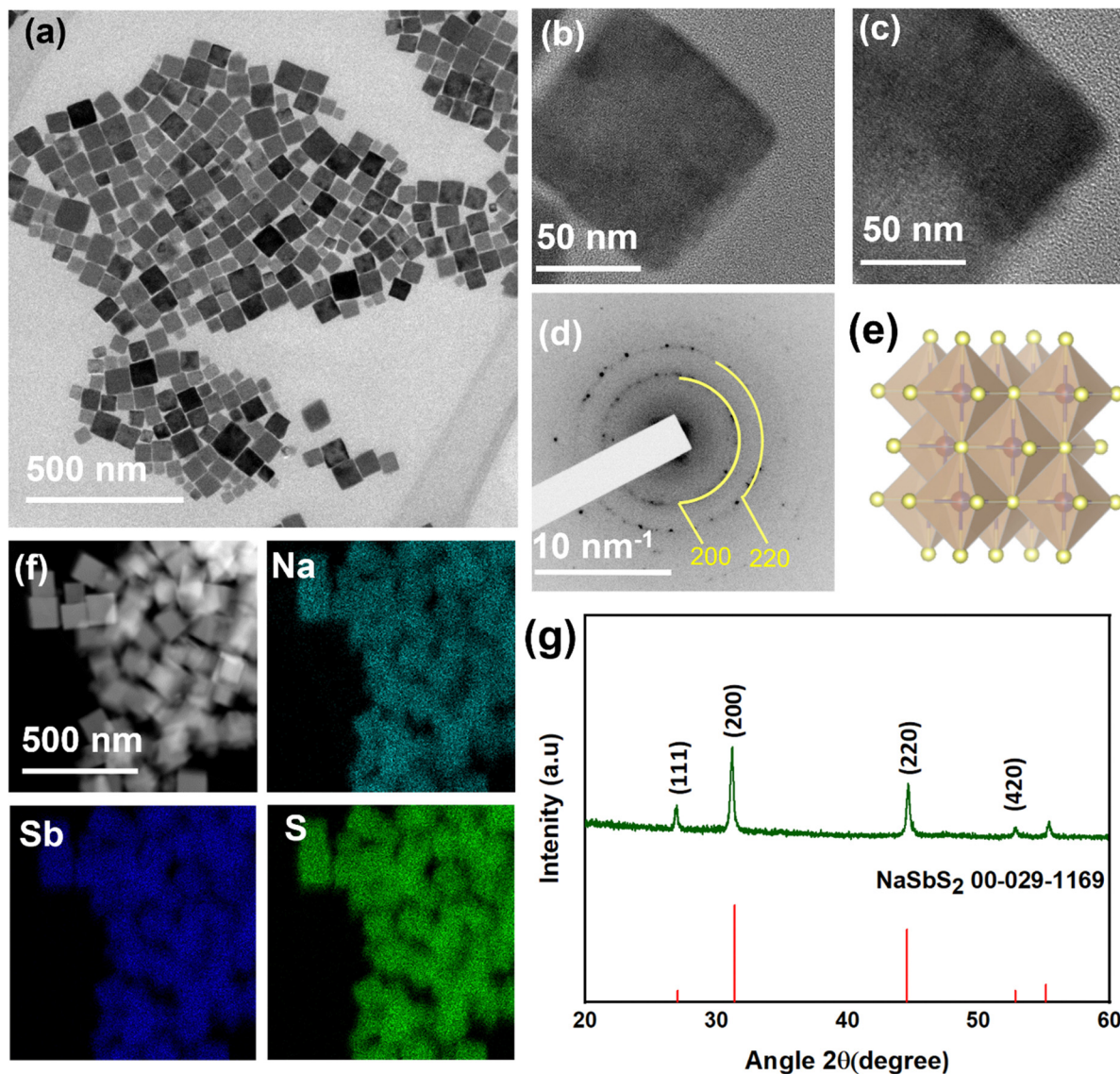
Fig. 1 TEM image (a) of NaSbS 2 NCs with (b and c) tilted TEM imaged at an angle of ±30° with (d) SAED and (e) crystal structure showing mixed cation sites of NaSbS 2 yellow (S), red (Na) and blue (Sb). (f) EDX elemental mapping for distribution of the three elements and (g) XRD pattern showing match to cubic phase NaSbS 2 (00-029-1169).
