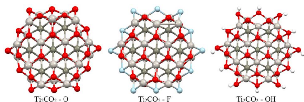
Fig. 9 Optimized structures of the studied \text{Ti}_2\text{CO}_2\text{-X} QDs with different edge functionalization (X = O, F, OH). Titanium, carbon, oxygen, fluorine, and hydrogen atoms are shown in light grey, dark grey, red, light blue, and white, respectively.
