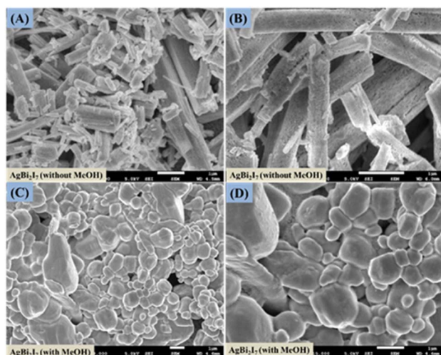
Fig. 2 FE-scanning electron microscopy images of \text{AgBi}_2\text{I}_7 perovskite without MeOH (A and B) and with MeOH (C and D).
