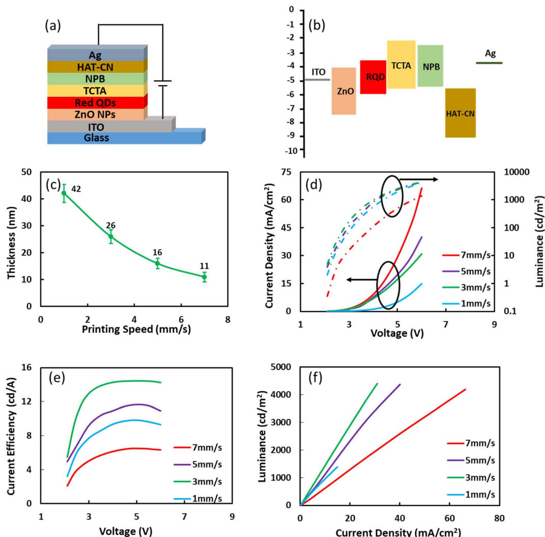
Fig. 3 (a) Schematic device architecture and (b) energy level alignment of PM bottom-emission QLED devices, (c) the thickness of the QD layer in the pixel at different printing speeds, (d) J-V-L characteristics, (e) current efficiency–voltage curves and (f) luminance–current density curves of QLEDs with various printing speeds.
