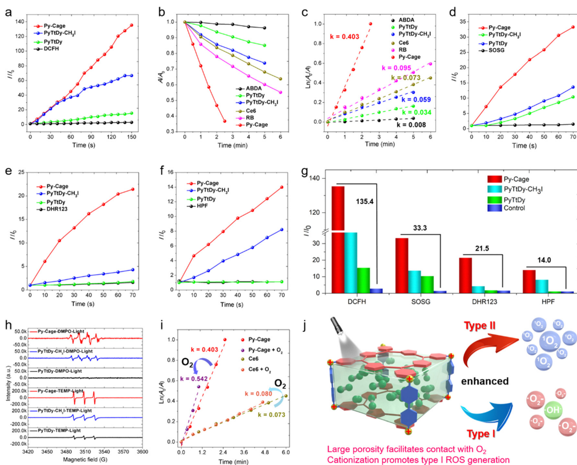
Fig. 3 (a) The ROS production of the Py-Cage, PyTtDy-CH 3 I, and PyTtDy (10 μg mL -1 ) was monitored under white light irradiation (white light, 20 mW cm -2 ) using DCFH as an indicator, respectively, the DCFH group was the blank control group under light conditions. (b and c) The 1 O 2 production of the Py-Cage, PyTtDy-CH 3 I, PyTtDy, Ce6, and RB was monitored under white light irradiation (20 mW cm -2 ) using ABDA as an indicator, respectively. The production of type II ( 1 O 2 ) and type I ( • O 2 - and • OH) ROS in the Py-Cage, PyTtDy-CH 3 I, and PyTtDy was monitored under white light irradiation using SOSG (for 1 O 2 ) (d), DHR123 (for • O 2 - ) (e) and HPF (for • OH) (f) as indicators, respectively. (g) Comparison of different ROS generation by the Py-Cage, PyTtDy-CH 3 I, and PyTtDy. (h) Comparison of the EPR results of the Py-Cage, PyTtDy-CH 3 I and PyTtDy under light conditions using DMPO (DMPO- • OH and DMPO- • O 2 - ) and TEMP (TEMP- 1 O 2 ) as ROS trapping agents, respectively. (i) Changes in 1 O 2 generation for the Py-Cage and Ce6 in an oxygen environment. (j) Schematic illustration of the enhanced ROS generation for cationic organic nanocage Py-Cage.
