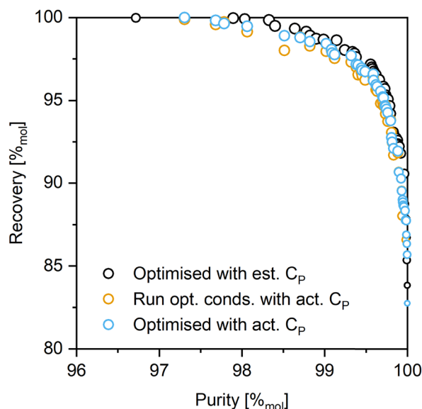
Fig. 7 Impact of performing optimisation with estimated C_p on F4_MIL-140A(Ce) for the 25.5% _{\text{mol}} \text{CO}_2 case under VSA conditions. Black symbols are optimisation undertaken with estimated heat capacity. Orange symbols are process performance based on the operating conditions determined with estimated heat capacity (previous case) but the measured/actual C_p is used. Blue symbols represent results if optimisation is carried out with the measured heat capacity directly (the same data from black symbols in Fig. 5F). The size of the symbols is proportional to the \text{CO}_2 working capacity.
