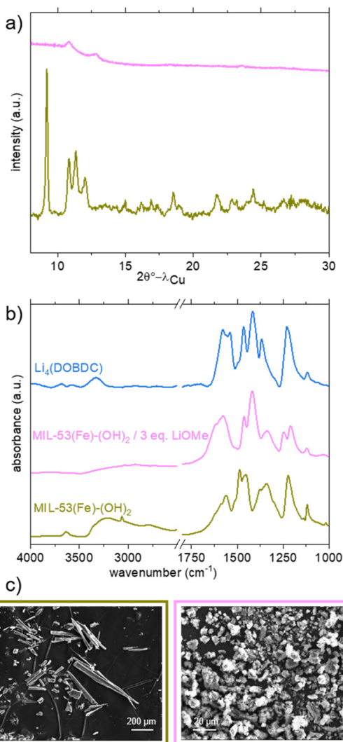
Fig. 5 Characterisation of \text{MIL-53(Fe)-(OH)}_2 and its lithiated product from LiOMe in MeOH/THF. a) PXRD patterns ( \lambda = 1.5406\text{ }\text{\AA} ); b) IR spectra; c) SEM pictures. Data related to dry \text{MIL-53(Fe)-(OH)}_2 , \text{Li}_4(\text{DOBDC}) and the lithiation product are shown in khaki, blue and pink, respectively.
