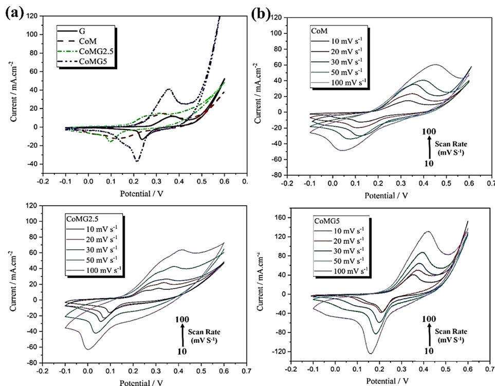
Fig. 6 The CV curves of (a) G, CoM, CoMG2.5, and CoMG5 at a scan rate of 10 \text{ mV s}^{-1} , (b) CoM, (c) CoMG2.5 and (d) CoMG5 electrodes at different scan rates ( 10 – 100 \text{ mV s}^{-1} ) in 6 \text{ M KOH} . Reproduced from ref. 143 with permission from Elsevier Ltd, Copyright 2021.
