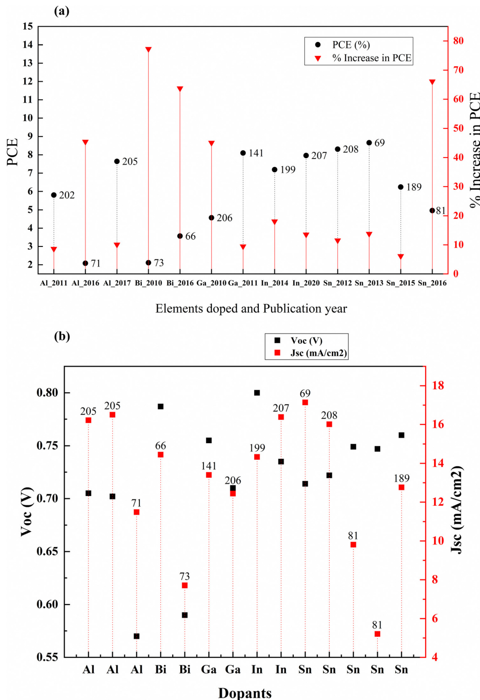
Fig. 23 (a) Percentage increase in PCE in post-transition metals with doping. (b) J_{sc} and V_{oc} of post-transition metals when doped into TiO_2 for DSSC fabrication. Data points are labelled with references.
