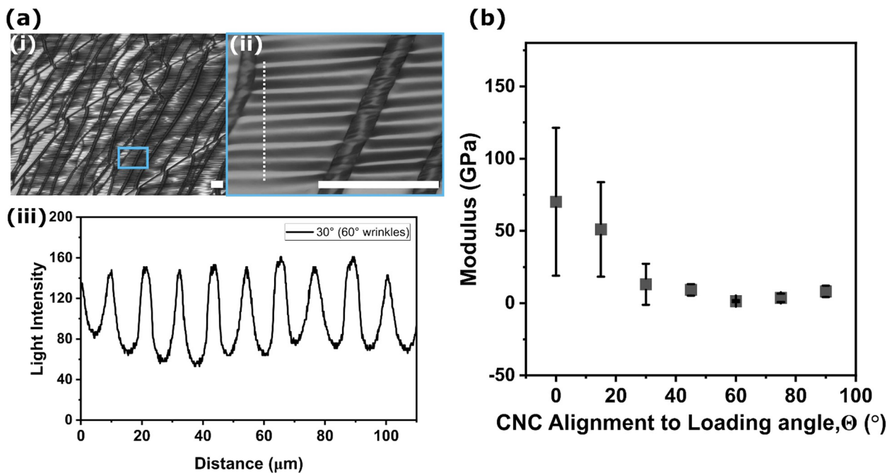
Fig. 4 (a) (i) The optical microscopy image of CNC film fracture morphology for the film aligned 30^\circ from the loading direction at approximately 25% strain. (ii) The magnified image of (i) where the blue square in (i) indicates the location. The scale bars are 100\ \mu\text{m} in both images. (iii) Wrinkling profiles measured in a line scan shown by the vertical dashed line in (ii). The wavelength of wrinkles was measured across 10 peaks in the profiles. (b) The modulus of CNC films with respect to alignment as calculated using the wrinkle wavelength and independent measurements of CNC film thickness and PDMS modulus.
