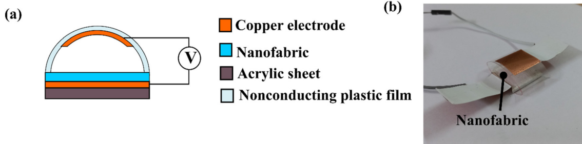
Fig. 2 (a) Schematic and (b) actual image of TENG.
