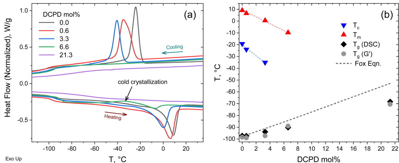
Fig. 4 Thermal properties of copolymers (a) DSC heating and cooling curves at 10 °C min -1 . (b) Thermal transitions as a function of DCPD content.
